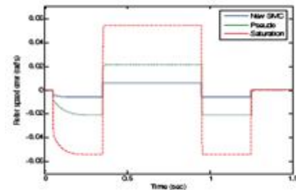
Fig.9. Rotor speed tracking error
