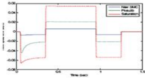
Fig.6. Rotor speed tracking error
