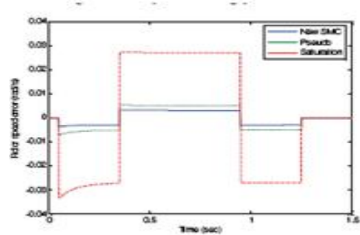
Fig.3. Rotor speed tracking error
