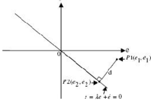
Fig.1. Derivation of signed distance
