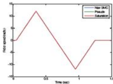
Fig.2. Rotor speed tracking performance
