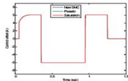
Fig.10. Control effort
